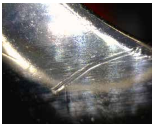
Deep Scratches on Ball from Debris Caused Seat Leakage
